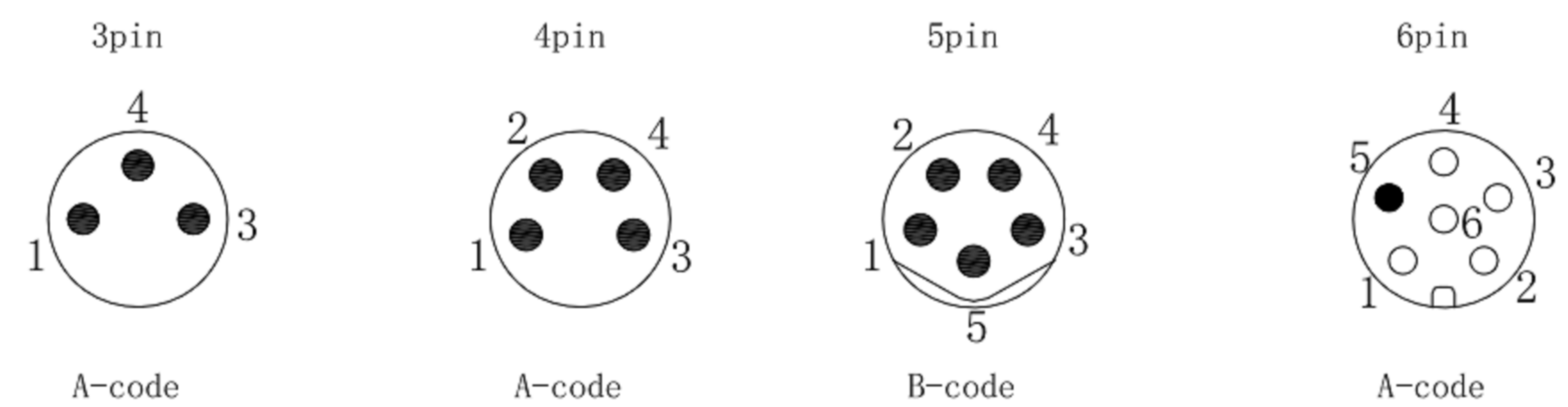
Pin assignment front view/针位分布前视图
